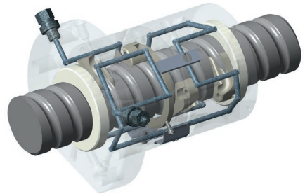
REFRIGERATED NUT
