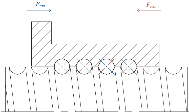
TMBS single non preloaded single nut, contact points
