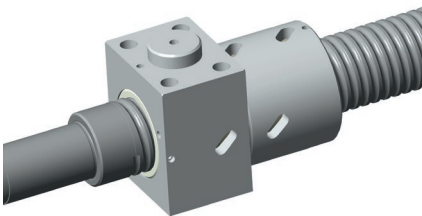
SPECIAL NUTS
