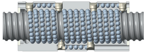
B-type recirculation system
