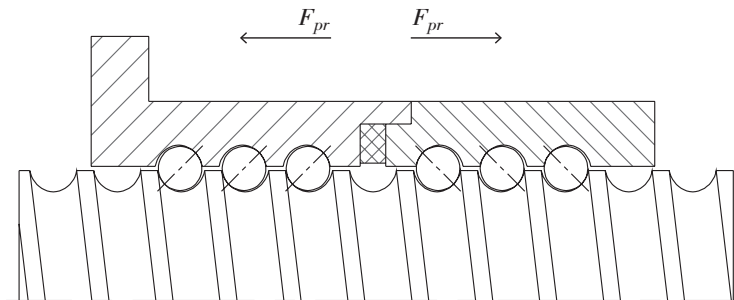
PRIME preloaded double nut, contact points
