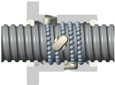
S-type recirculation system
