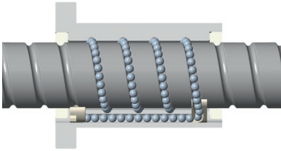
U-type recirculation system
