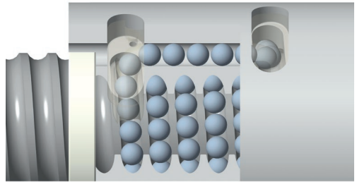
B-type recirculation
