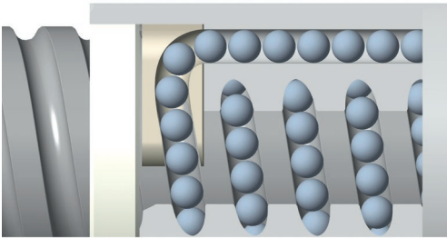
U-type recirculation
