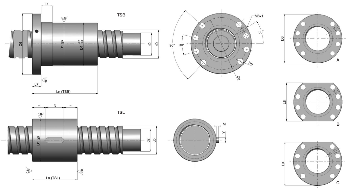
HIGH LOADS Single Nut
