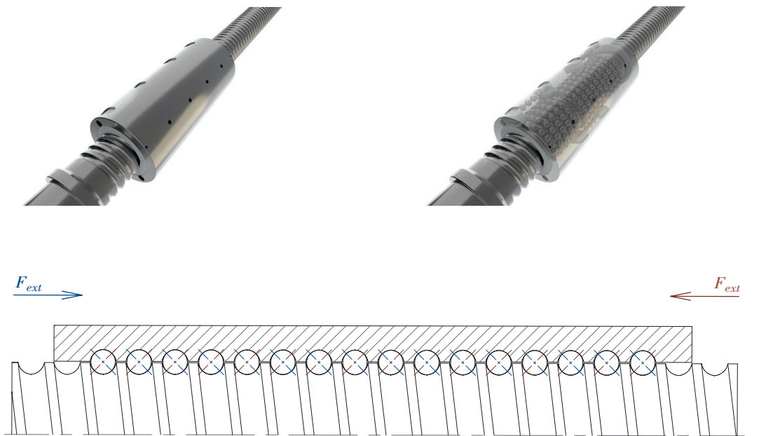
Loading Nut, contact points
